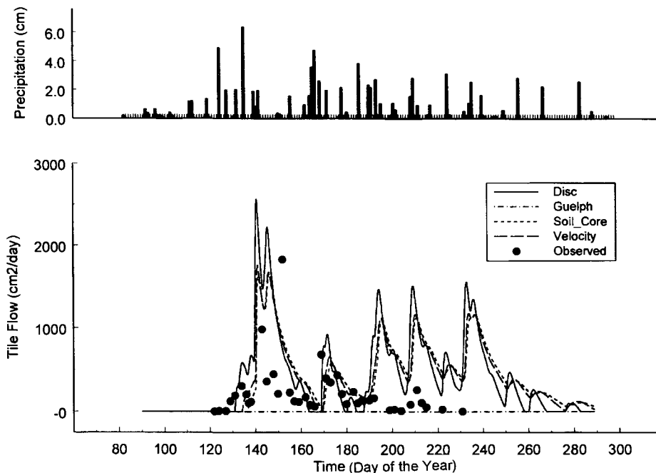
Fig. 5. Comparison of observed and predicted tile flow during the crop growing season of 1990 at the field site using different K_s . Also shown are precipitation data at a nearby weather station during the same period.
