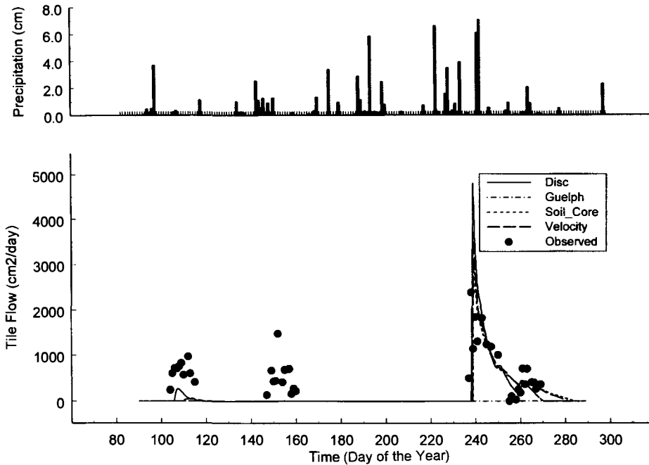
Fig. 4. Comparison of observed and predicted tile flow during the crop growing season of 1987 at the field site using different K_s . Also shown are precipitation data at a nearby weather station during the same period.
