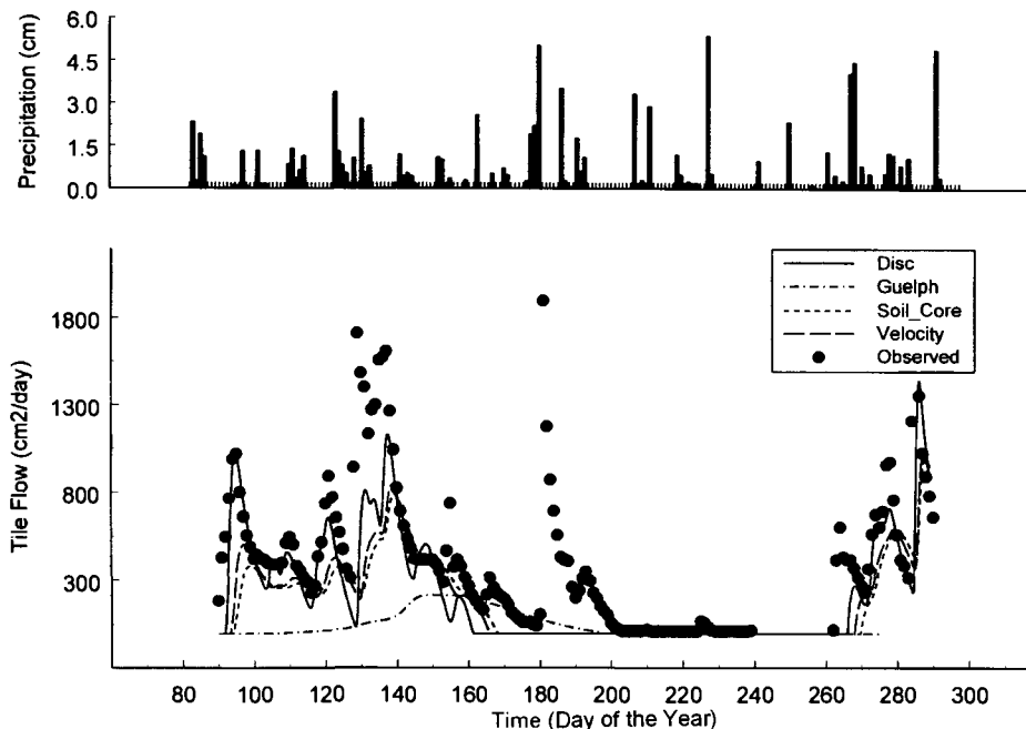
Fig. 3. Comparison of observed and predicted tile flow during the crop growing season of 1986 at the field site using different K_s . Also shown are precipitation data at a nearby weather station during the same period.
