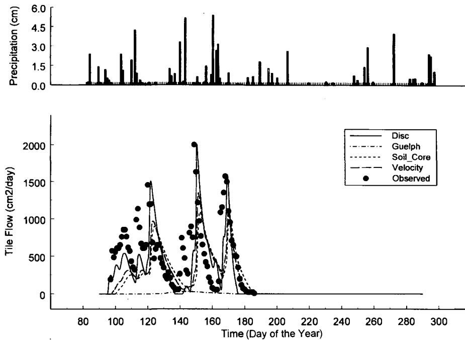
Fig. 2. Comparison of observed and predicted tile flow during the crop growing season of 1984 at the field site using different K_s . Also shown are precipitation data at a nearby weather station during the same period.
