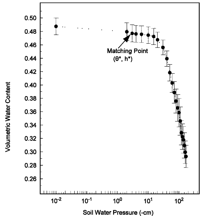
Figure 4. Error bar (arithmetic mean and standard error) plot of the (field-averaged) soil water retention ( \theta - h ) function for the surface horizon measured in the laboratory. Turning point at 30 cm indicates the bubbling pressure.
