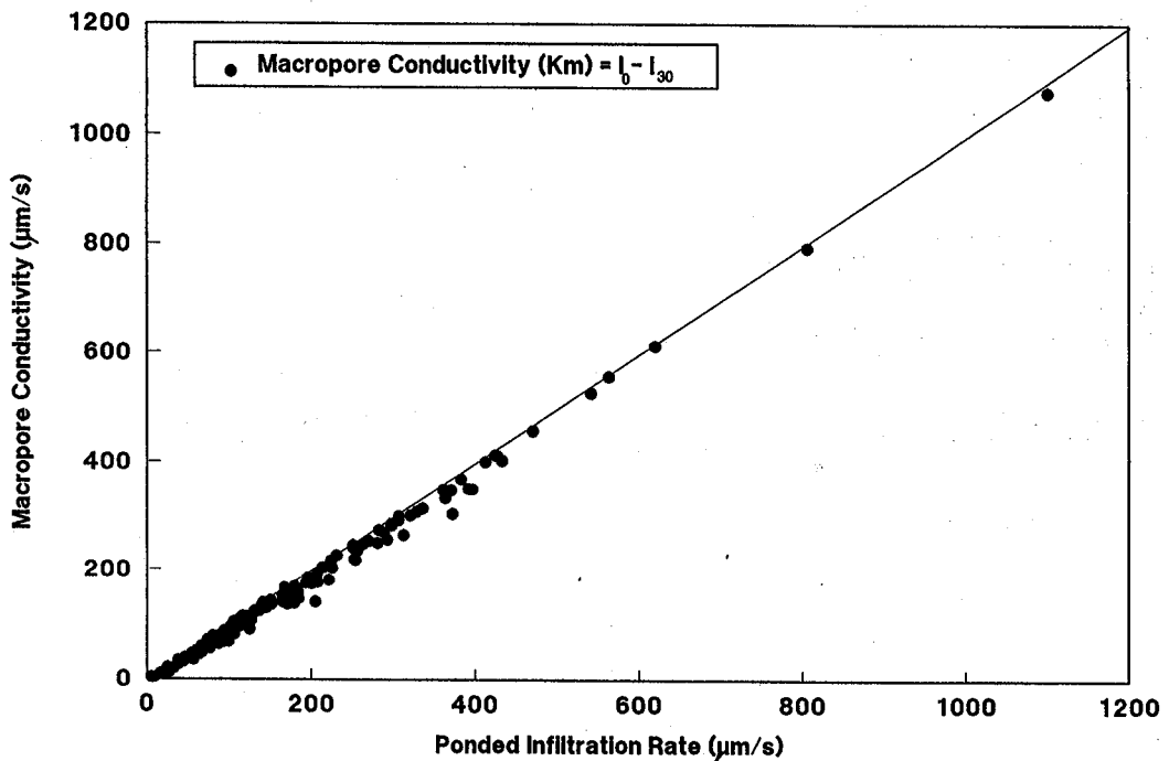
Fig. 4. Correlation between ponded infiltration rate ( I_0 ) and macropore conductivity ( K_m ) under corn row position.
