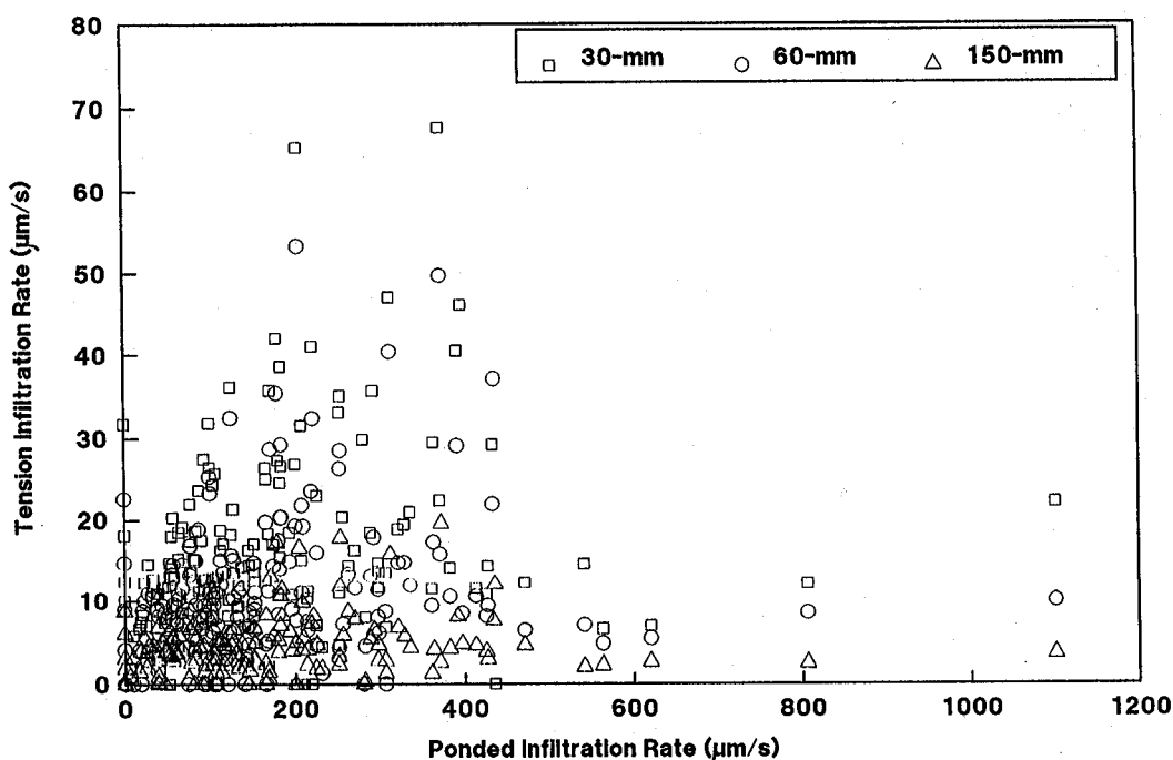
Fig. 3. Scatter plot of ponded infiltration rate ( I_0 ) versus tension infiltration rates ( I_{30} , I_{60} , I_{150} ) under corn row position indicating little correlation.
