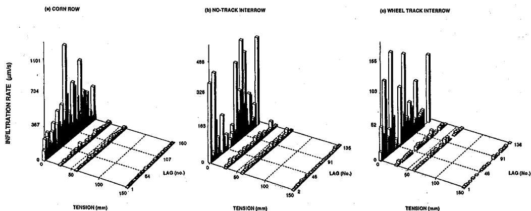
Fig. 2. Spatial distribution of infiltration rate ( \mu\text{m/s} ) at 0, 30-, 60-, and 150-mm tensions along the transect under (a) corn row, (b) nontrafficked interrow, and (c) trafficked interrow positions. Blank spaces in between measurements indicate missing data.
